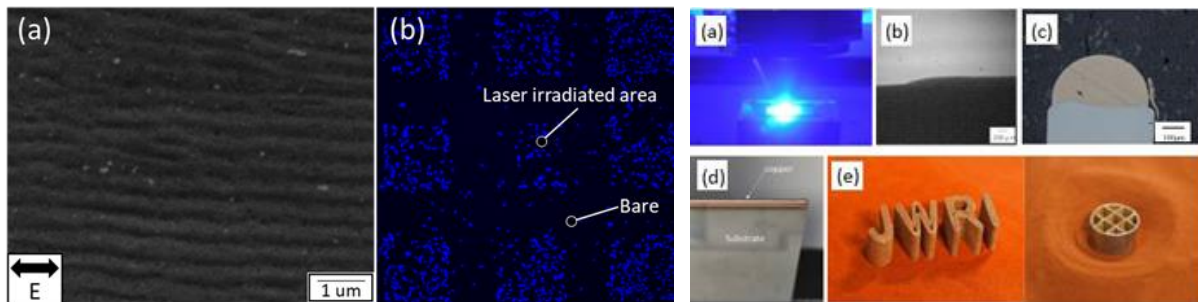
PMMA film surface after femtosecond laser irradiation. (a) SEM image with periodic nanostructures oriented to the direction perpendicular to the laser polarization vector (The period of the periodic nanostructure is about 230nm) on PMMA film surface. (b) Fluorescence microscope image of cell cultivation test. Cells adhered to the periodic nanostructures surface rather than bare surface.
