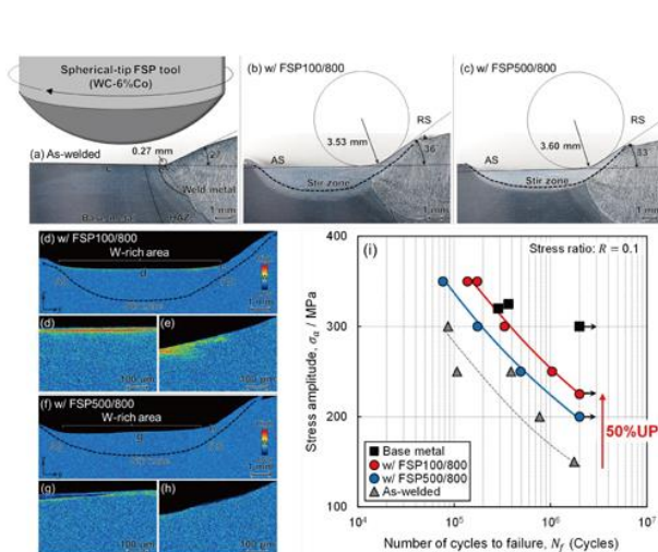
Geometry modification and W-rich layer formation for weld toe of high-strength low-alloy steel joints using friction stir processing (FSP) with spherical-tip WC tool, resulting in fatigue strength improvement.
