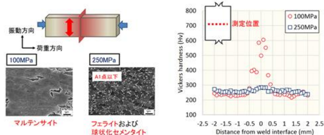
SEM microstructures and Vickers hardness along the central axis of LFWed joints.
